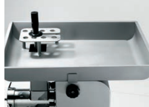
Tramoggia super Lager tray super
