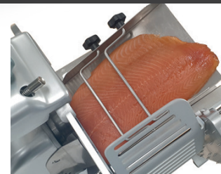
Slitta pesce Poseidon per piatto Uniko Poseidon fish cutting for Uniko hopper
